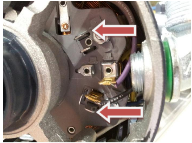
Line connection spades for L1, Neu (arrow 1 & 2)
