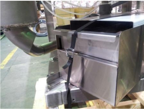
Front view of Scrap Box in transport position
