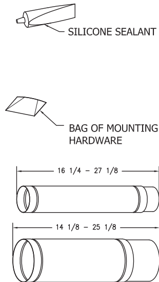
DIRECT VENT-AIR INTAKE KIT H PART NO. 239-42514-00 (OPTIONAL) ABOVE TUBE LENGTHS SUPPLIED WITH HEATER
