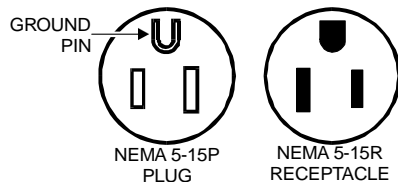
Fig. 3 Power Supply Plug
