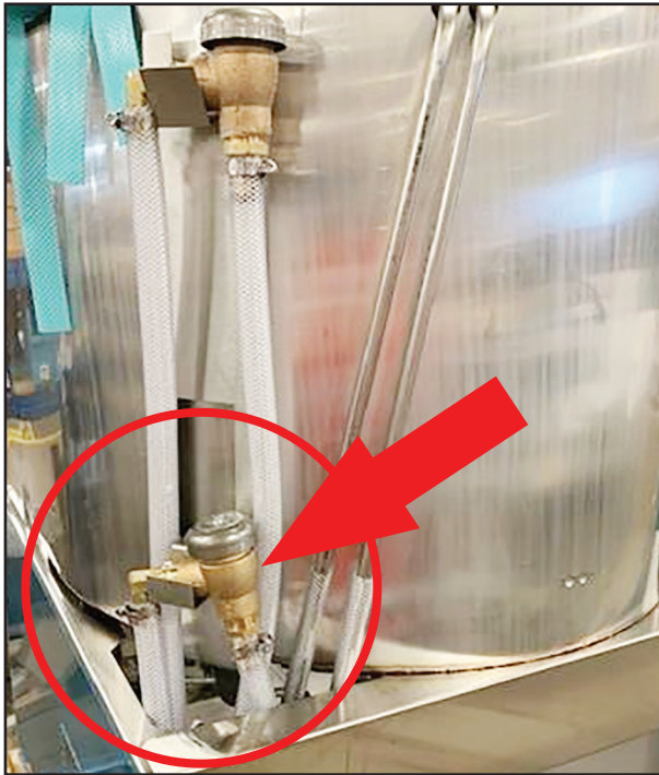
Upper piping configuration with vacuum breaker beginning with S/N G200325482.
