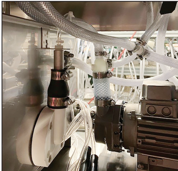
Lower piping configuration beginning with S/N G200325482.
