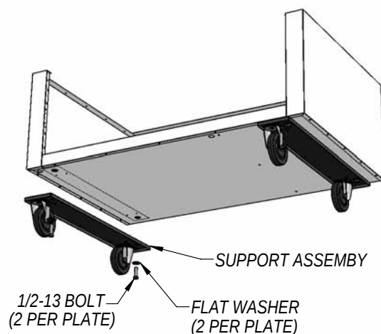
FIGURE 14: Caster Support Plates
