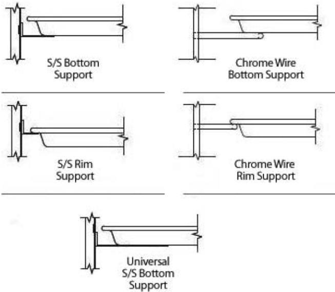
FIGURE 11: Pan Slide Assembly Configurations
