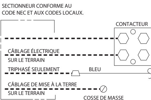
Figure 6 – Raccords de conduite
