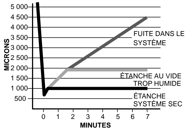
Figure 4 – Courbe de vide
