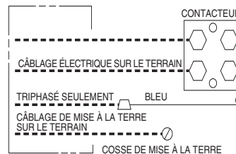
Figure 9 – Raccords de conduite
