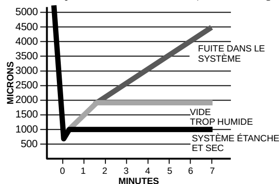
Figure 7 – Courbe de vide
