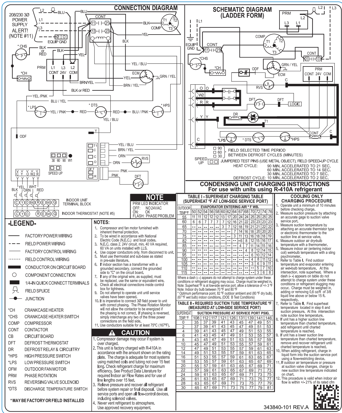
Fig. 4 – Wiring Diagram — Model size 60 - 208/230-3
