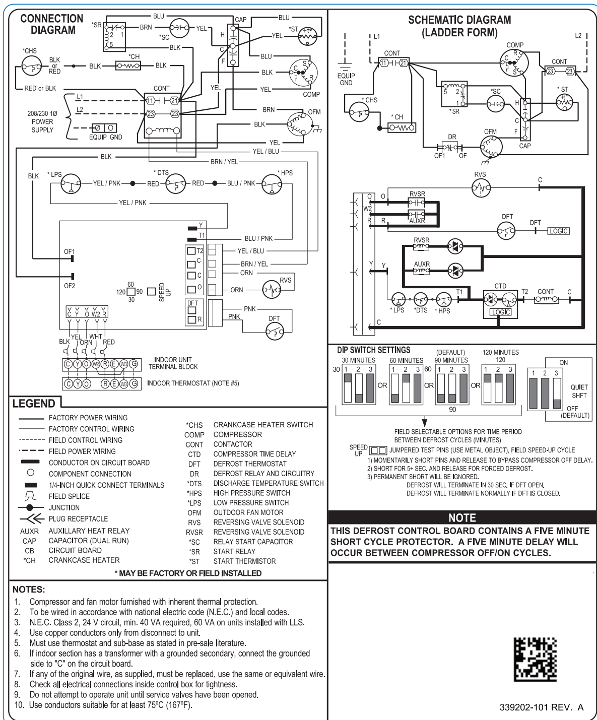
Fig. 1 – Wiring Diagram — Model sizes 18, 24, 30 36, 48 - 208/230-1
