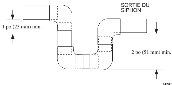
Figure 8 – Siphon de condensat
