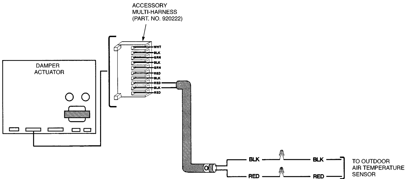
Fig. 4 — Outdoor Air Sensor Damper Board Wiring
