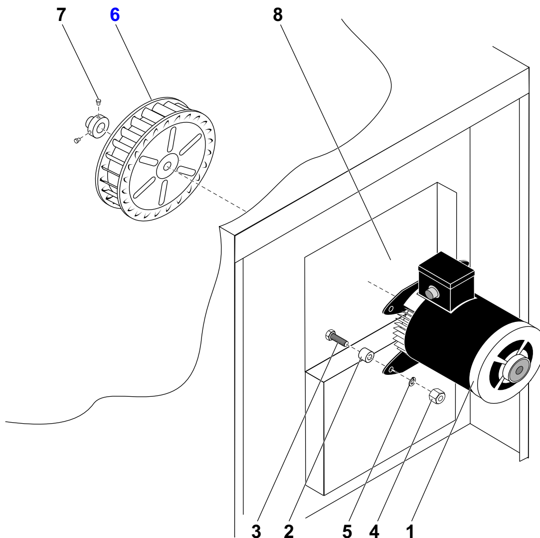
Figure: PL-3 Rear Mounted Fan Motor & Heaters
