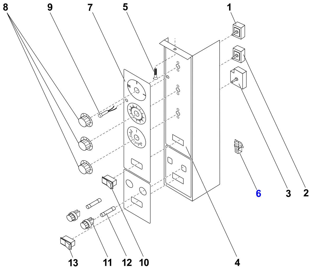
Figure: PL-8 “ZX” Control Panel Assembly 6/13 & 5/9 Series
