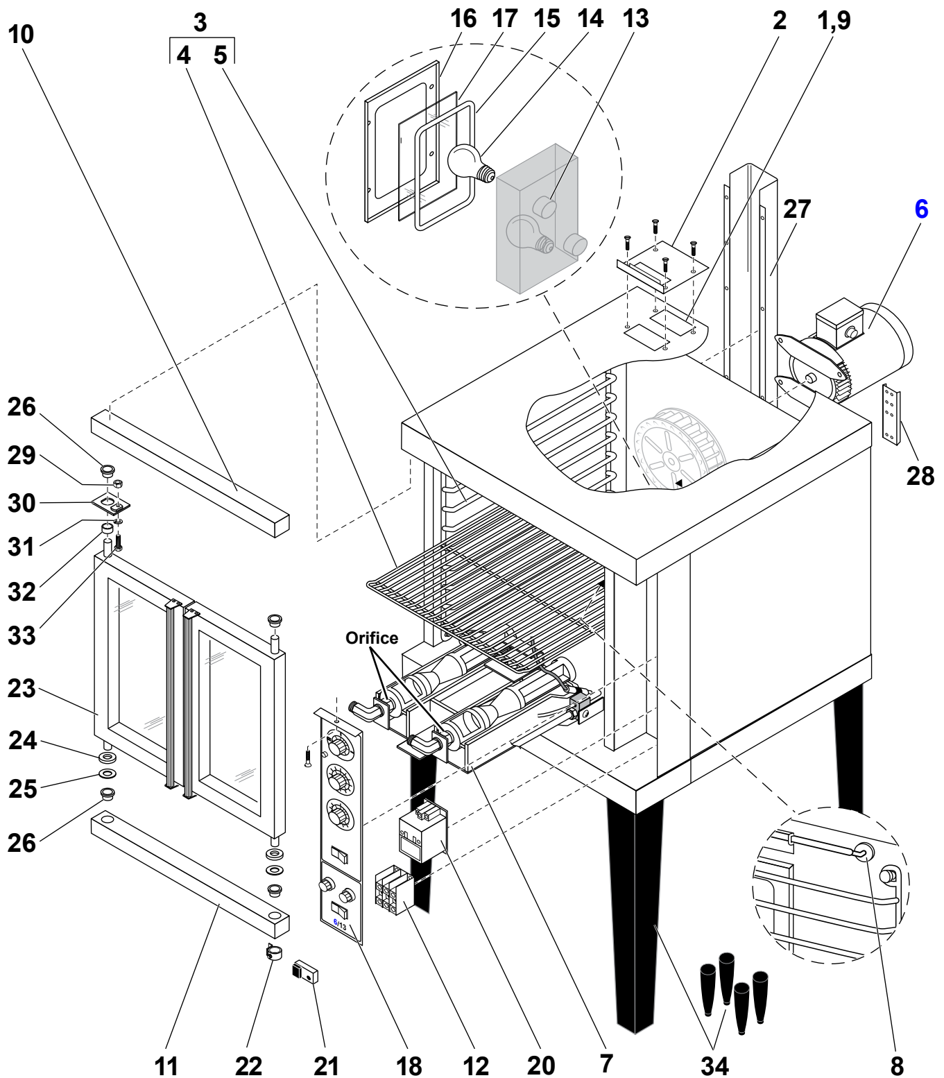
Figure: PL-1 6/13 The Oven, "E" Series, Double Door Units
