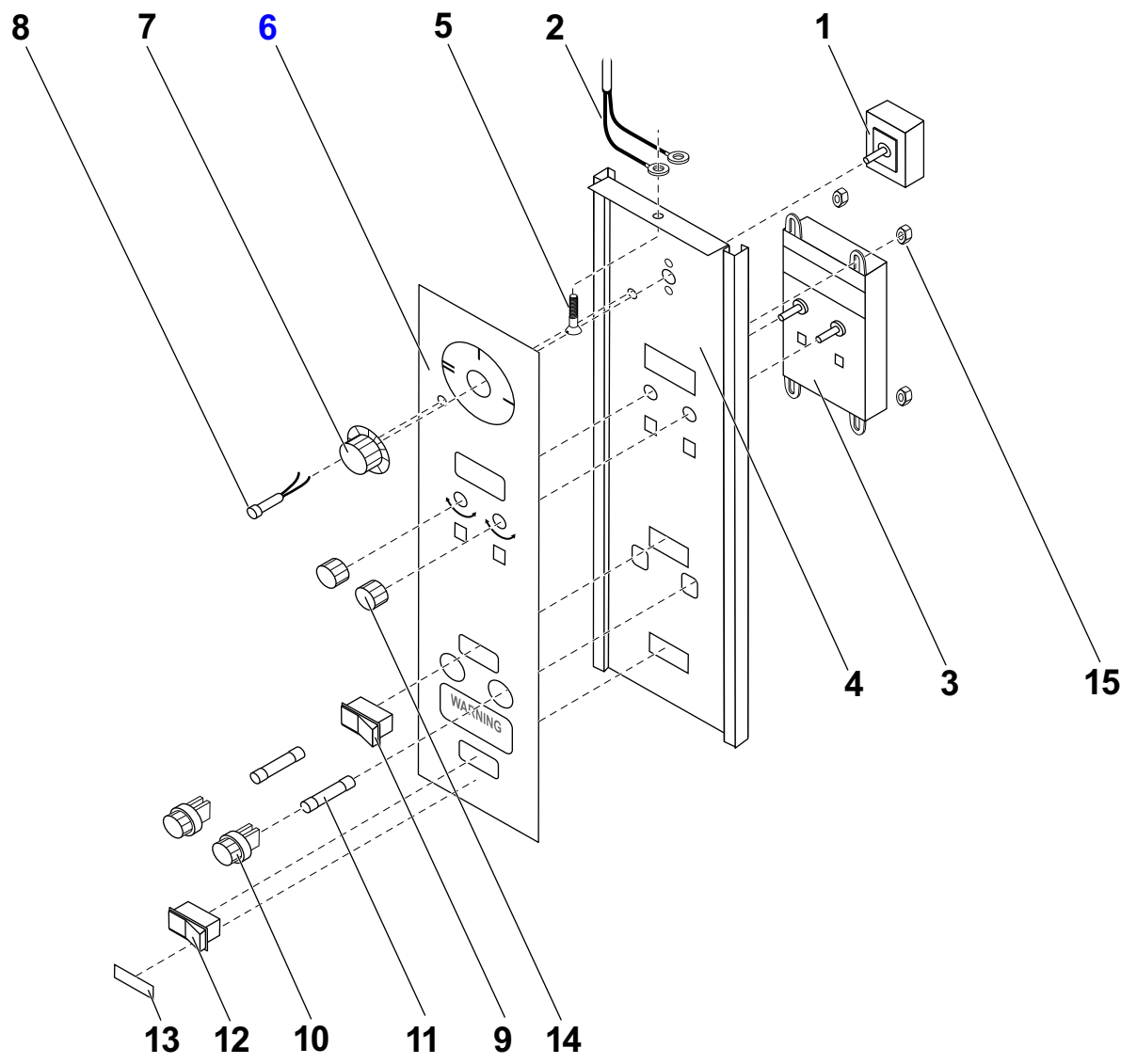
Figure: PL-4 X Control Panel Assembly for 6/13 Series
