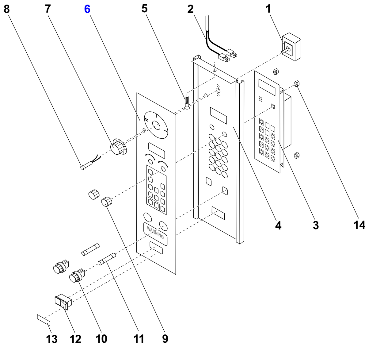
Figure: PL-6 “Z” Control Panel Assembly 6/13 Series
