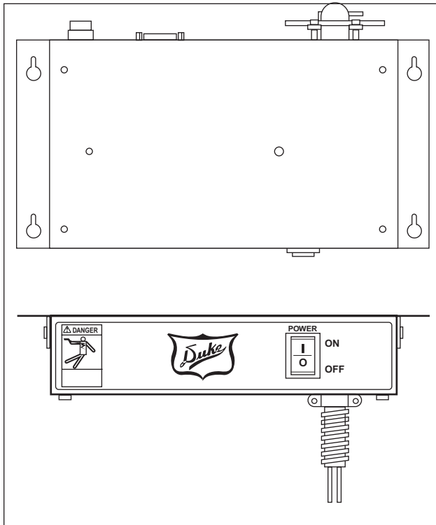
Figure 8. Relay Box
