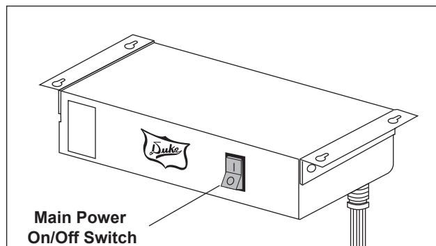
Figure 4. Relay Box
