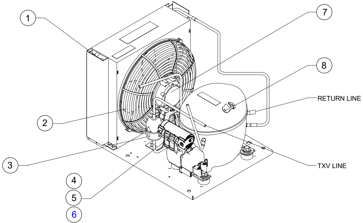
516828 Emerson Condensing Unit, 208/230V, 60Hz, R-290 refrigerant
