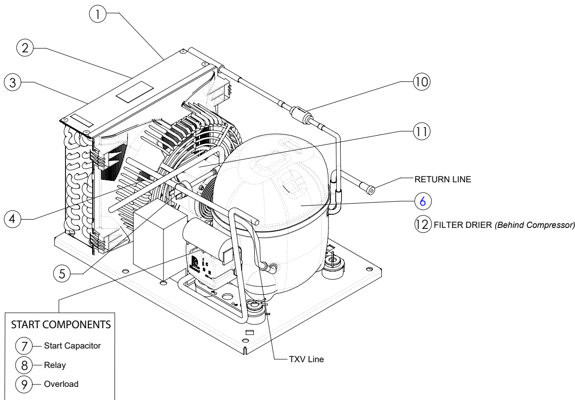
516817 Tecumseh Condensing Unit, 220/240V, 50Hz, R-290 Refrigerant
