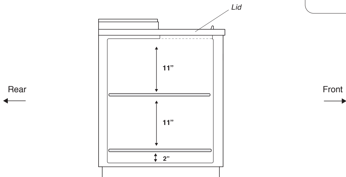
Side View
