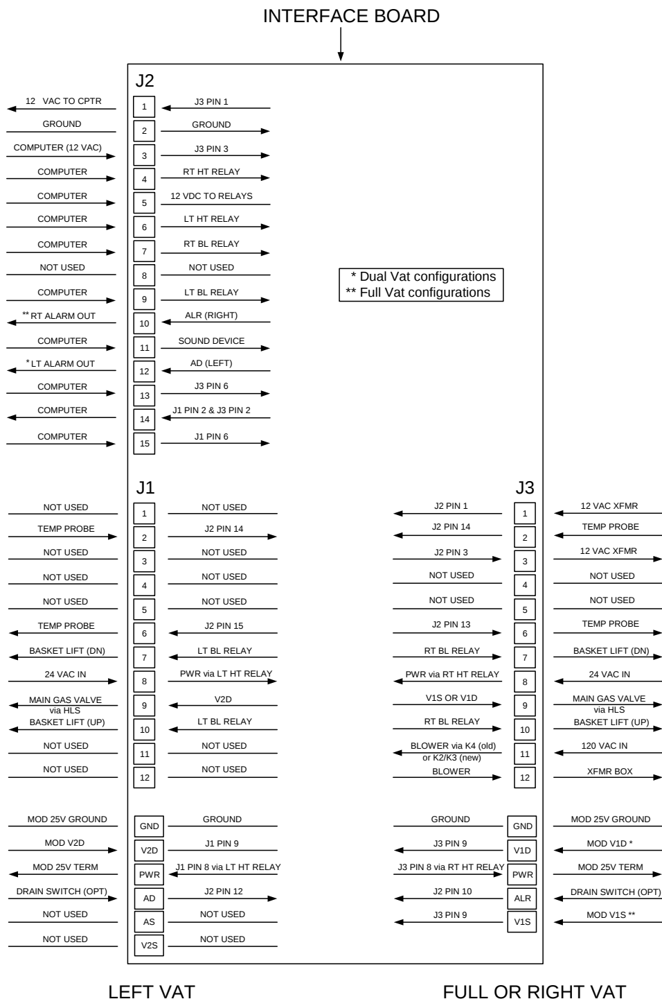
CURRENT FLOW THROUGH INTERFACE BOARDS 806-3398 AND 106-0386 (H50 APPLICATION)
