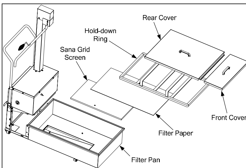
Filter assembly.
