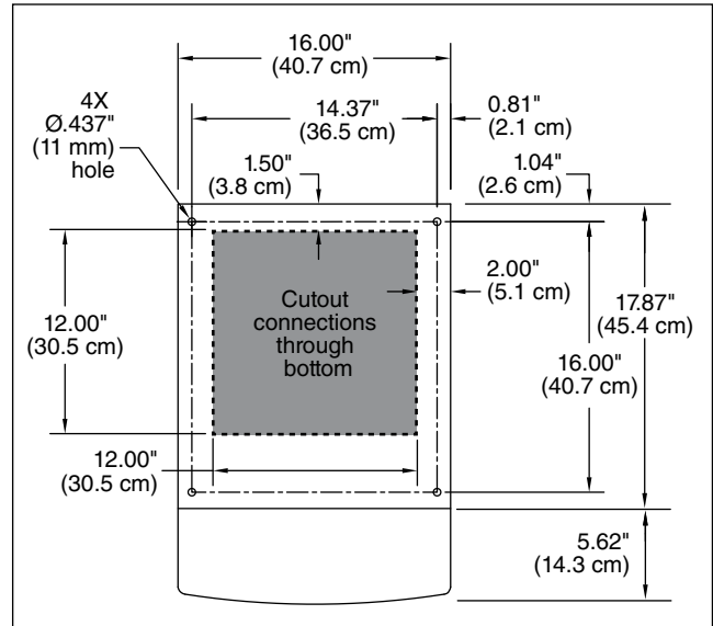
Fig. 2 - Bottom exiting utilities (countertop units)
