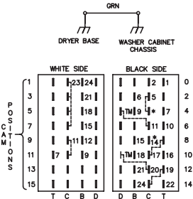
TERMINAL POSITION CHART (END VIEW)
