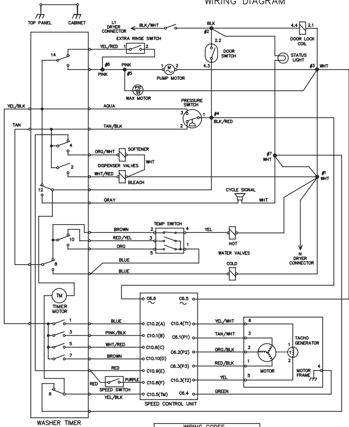
WIRING DIAGRAM
