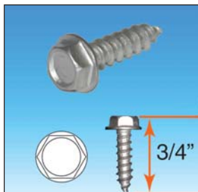
S8X10HXWHCTS Hex Washer Head Screw For "J"Hook
