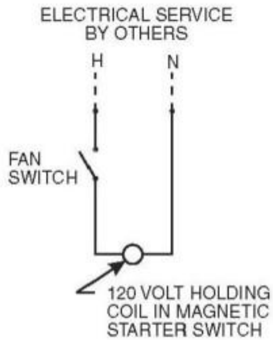
Figure 6-1-1 Typical Exhaust Fan Switch Wiring
