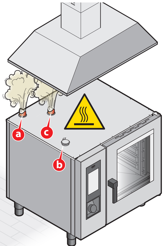
modelli gas gas models
