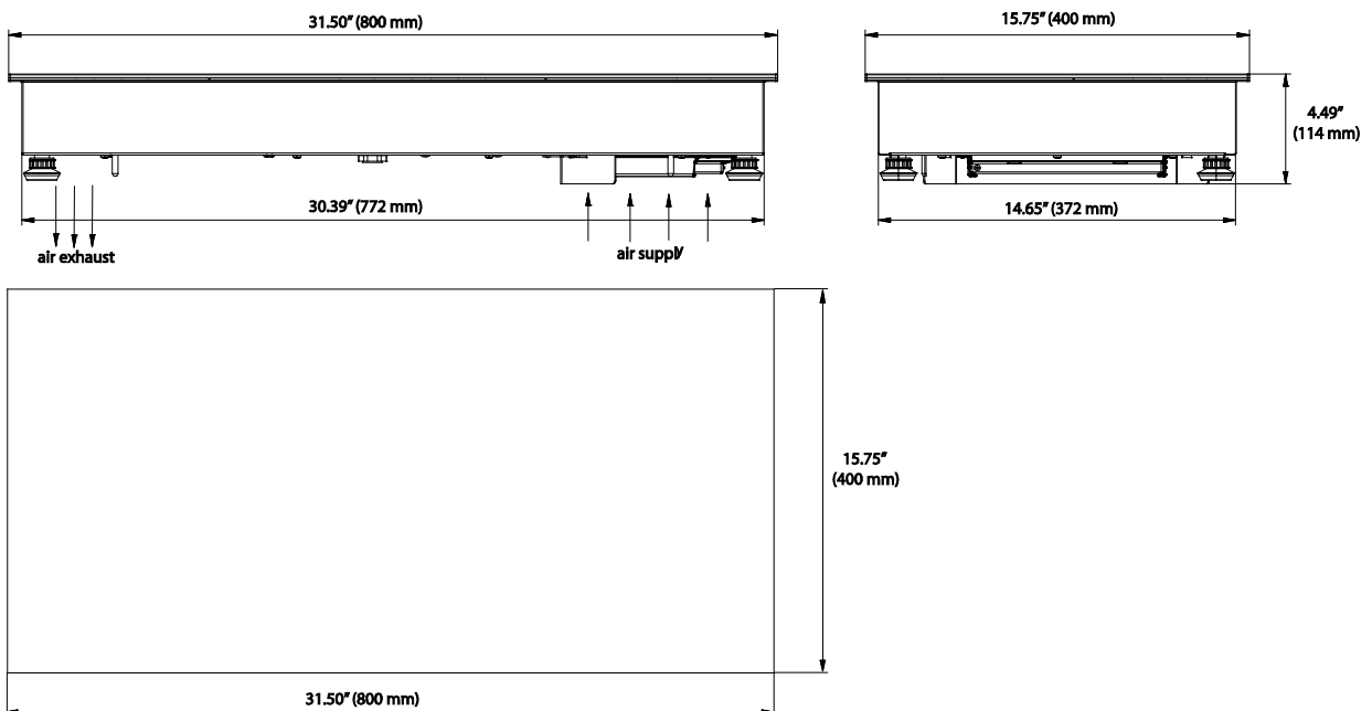
Dimensions: RTCSmp Tabletop Hold-Line HO1500
