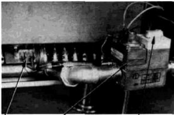
PILOT BURNER COMBINATION GAS CONTROL VALVE SELECTOR KNOB
