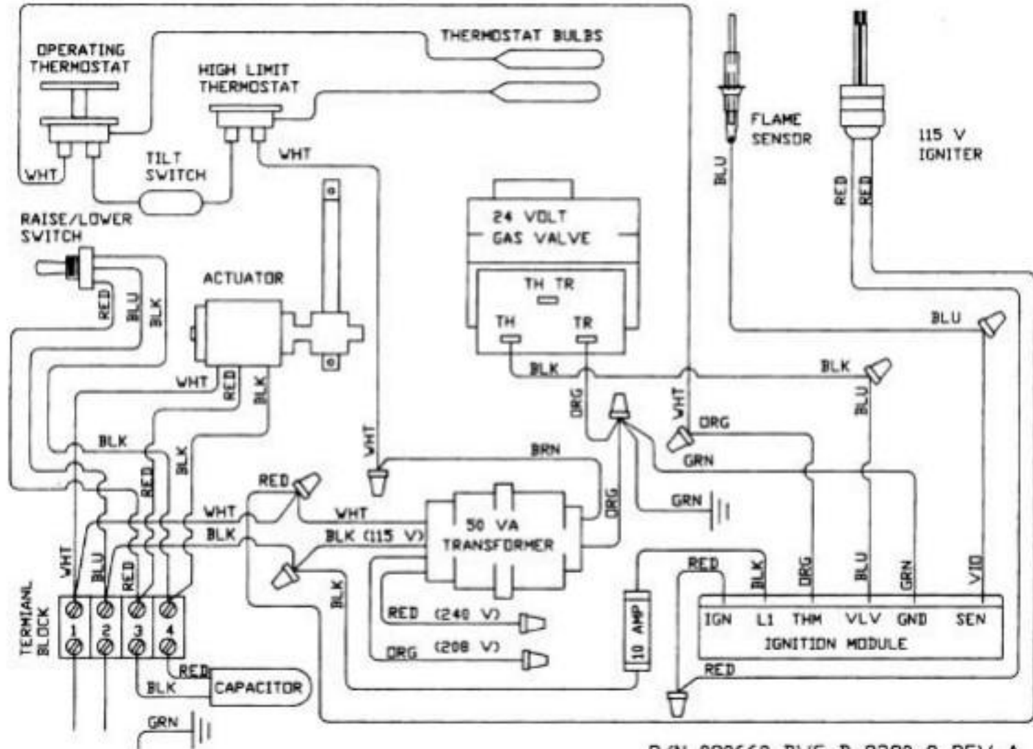
Wiring Diagram for units built after April, 1991
