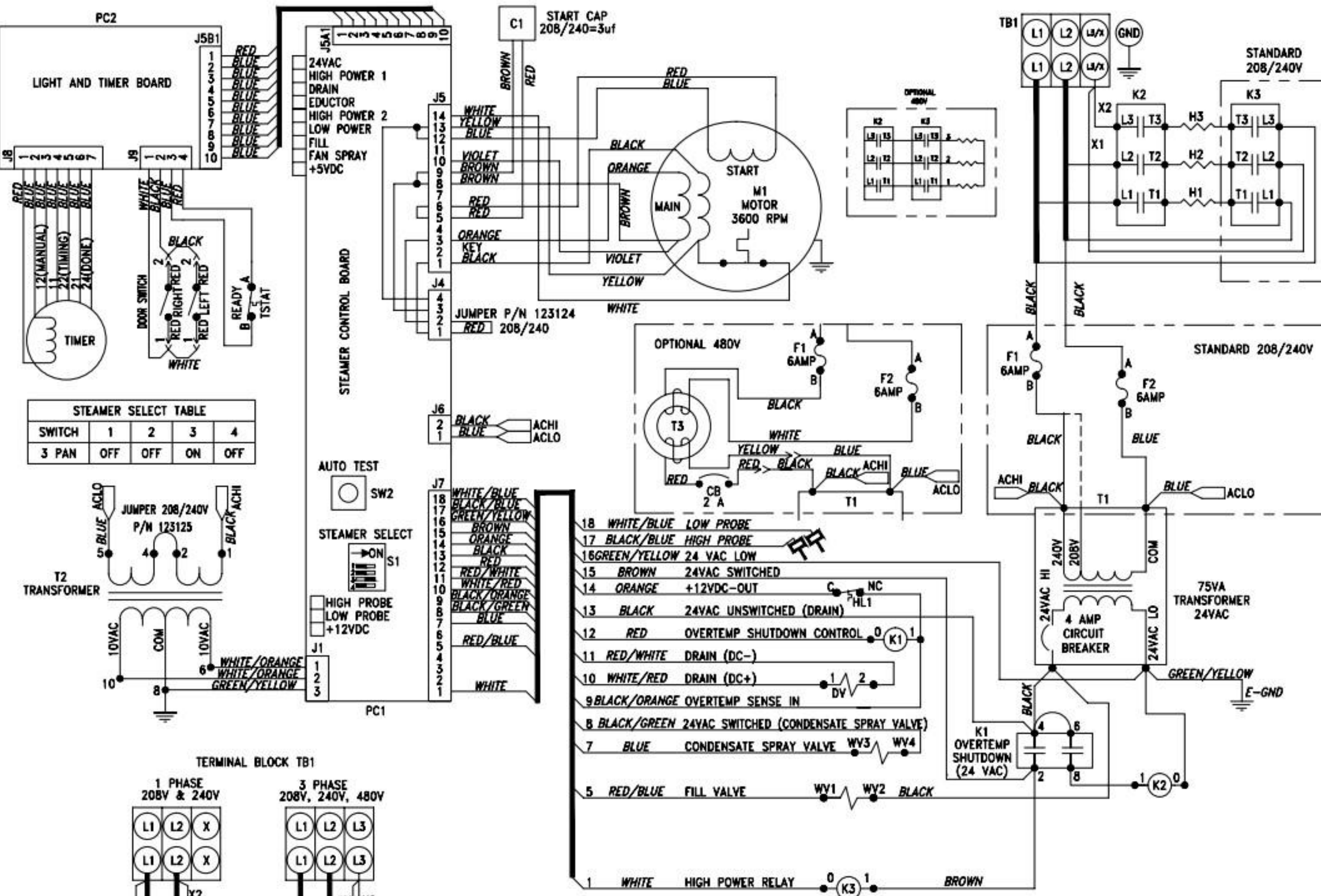
3 PAN WIRING DIAGRAM P/N 148114 REV F
