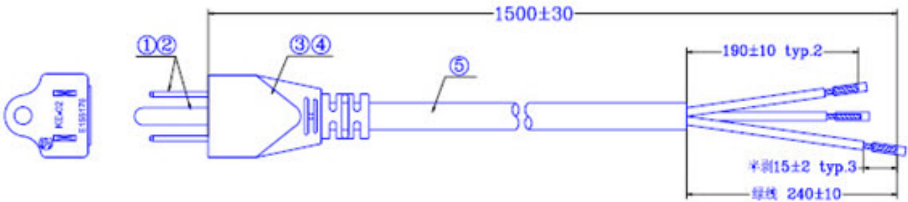
Power Cord 990167500
