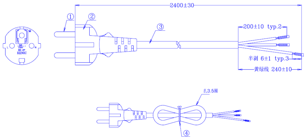
Power Cord 990167370
