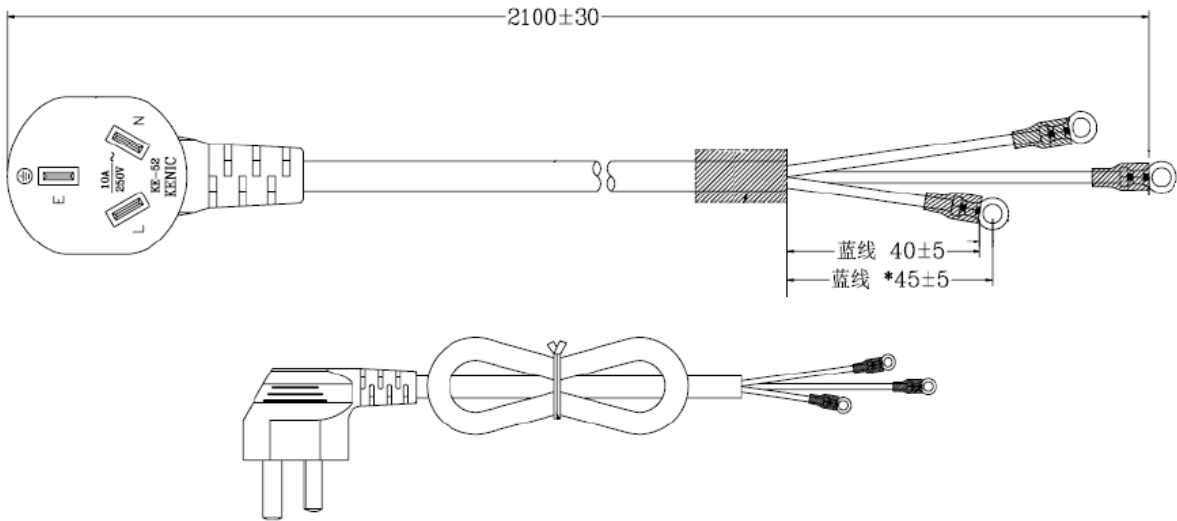
Power Cord 990310800
