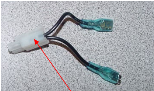
Switch Adaptor 990088900
