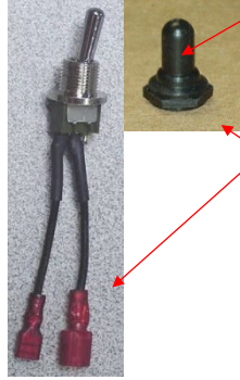
Toggle Switch, Boot and Lead Wires – Sub-Assembly 990083600
