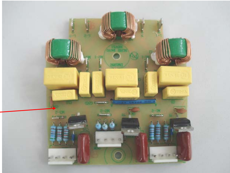
RFI Board 990050500
