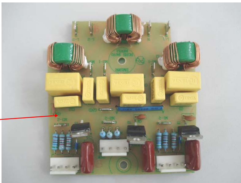
RFI Board 990050500
