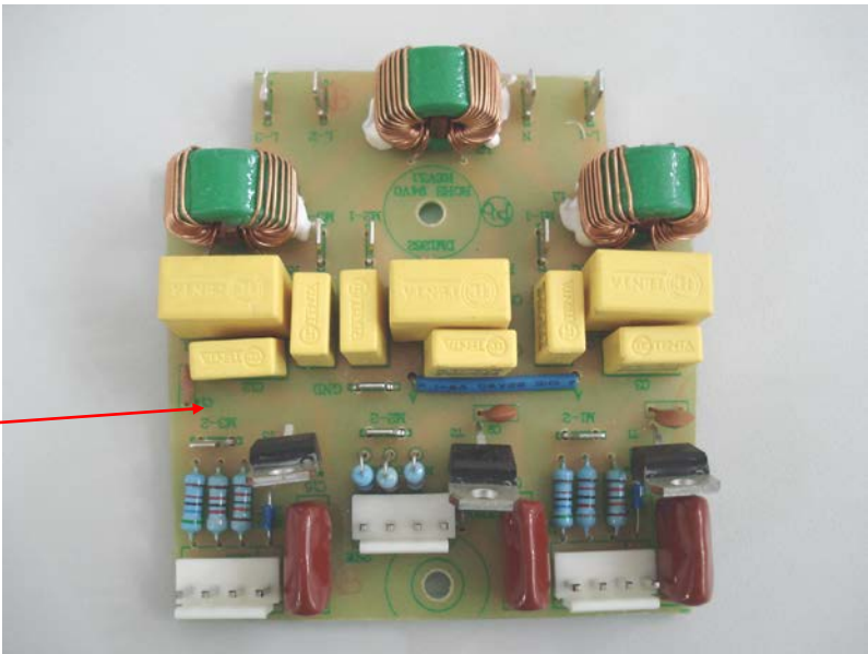
RFI Board 990050500
