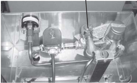
SAFETY VALVE
