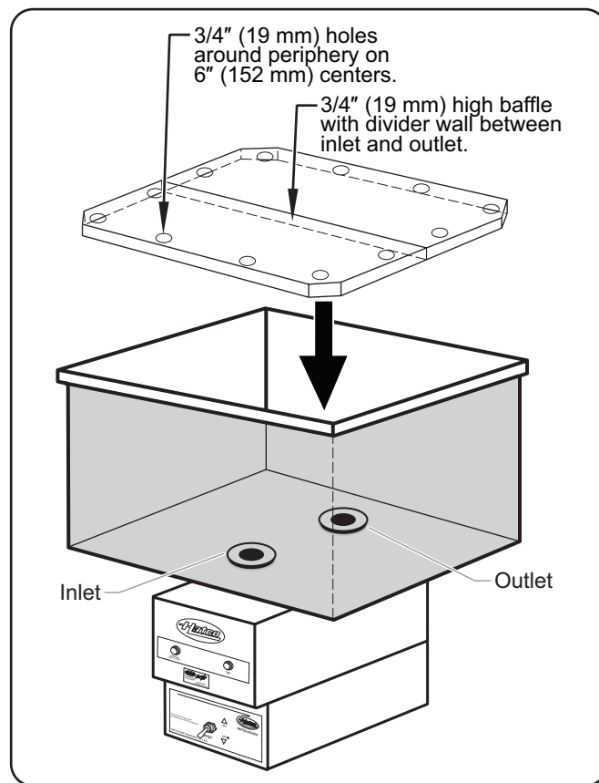
Water Baffle Installation (FR Models)
