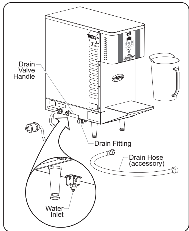
AWD-12 Installation
