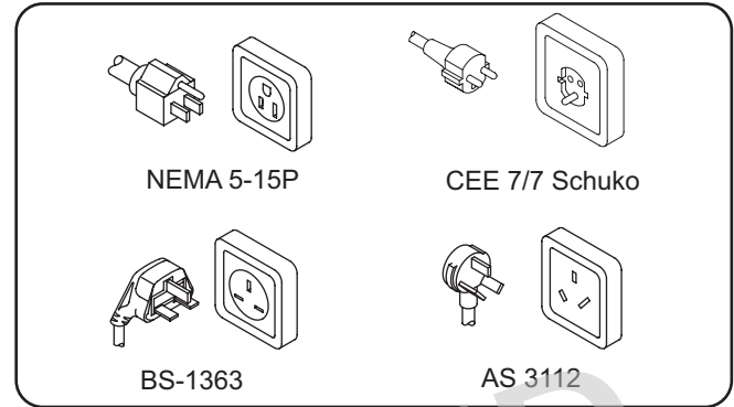
Plug Configuration
