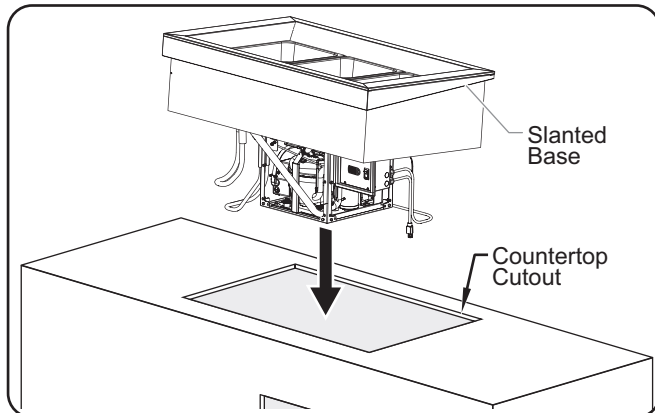
Installing a Slanted Base
