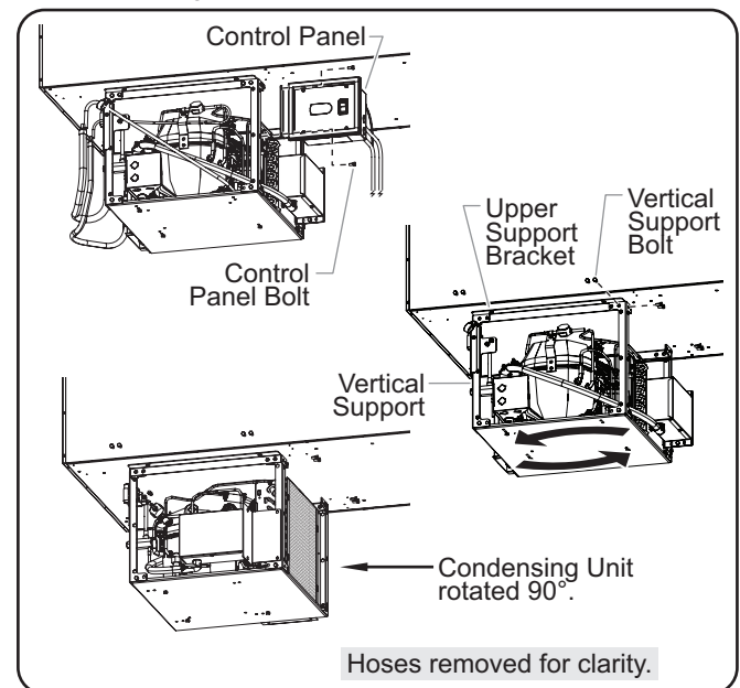
Rotating the Condensing Unit
