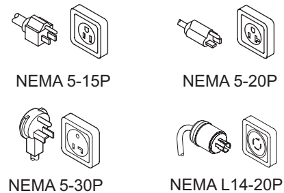
Plug Configurations
