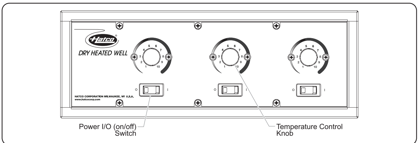
Control Enclosure
