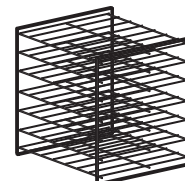
7-Shelf Multi-Purpose Rack Shelves 1 & 5 Rack Opening: 2-1/2" (63 mm). NOTE: Shelf 1 is the bottom shelf. Shelves 2, 3, 4 & 6 Rack Openings: 2-3/4" (69 mm) Shelves 2, 3, 4, 6, & 7 are removable.
