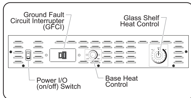
Controls for GRHW-1SGD and GRHW-1SGDS (GRHW-1SGDS controls shown)
