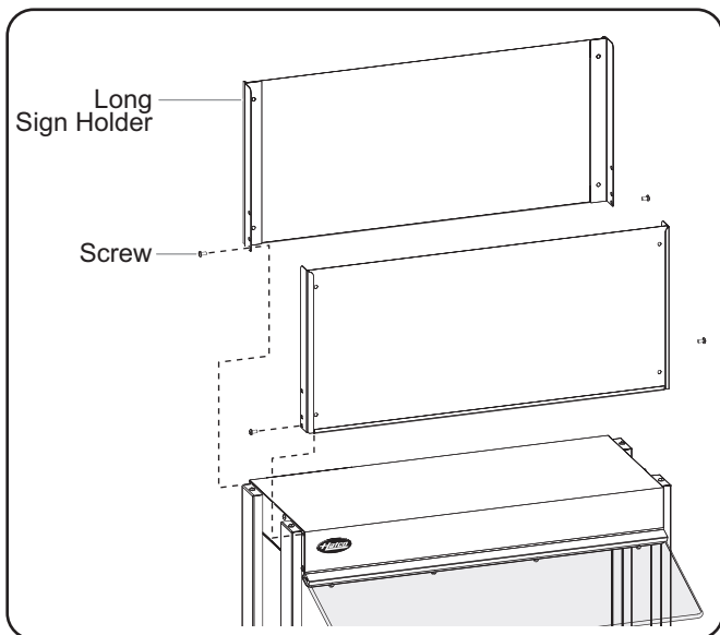
Installing the Front and Rear Long Sign Holders
