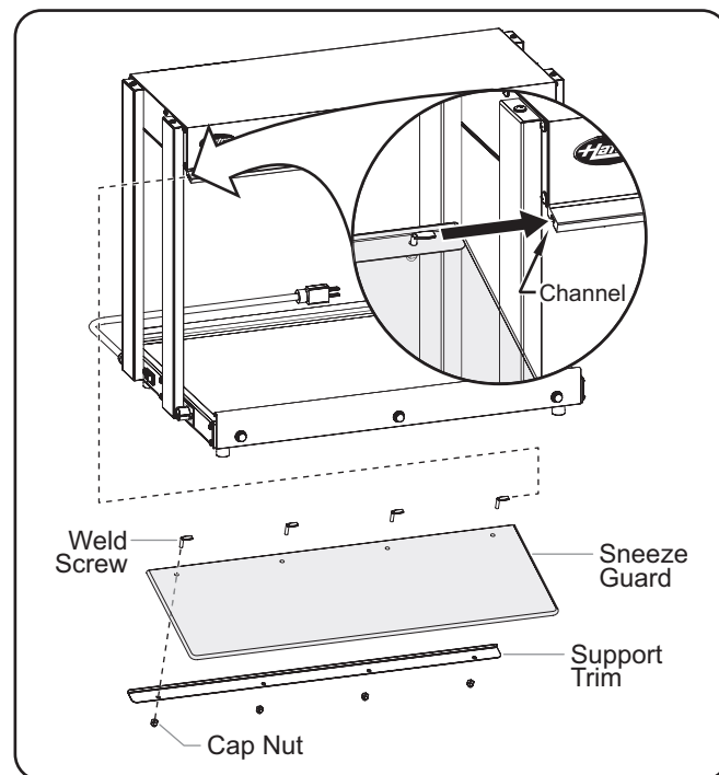
Installing a Sneeze Guard (GRHW-1SG model shown)
