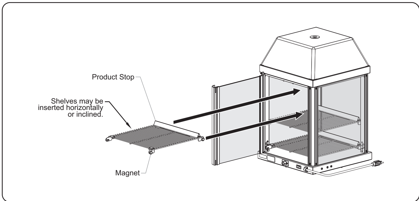
Shelf Installation
