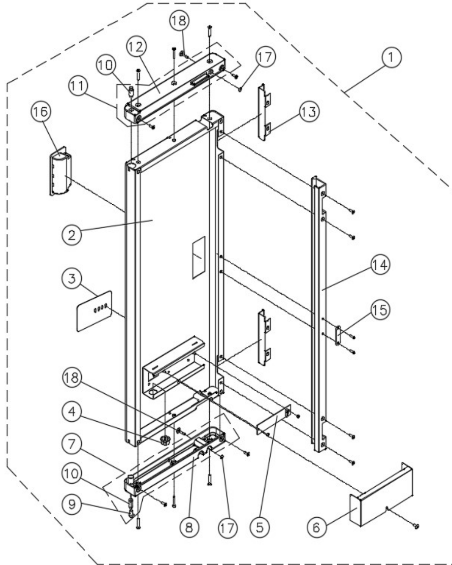
[ FRONT PANEL ASSY(R) ]
