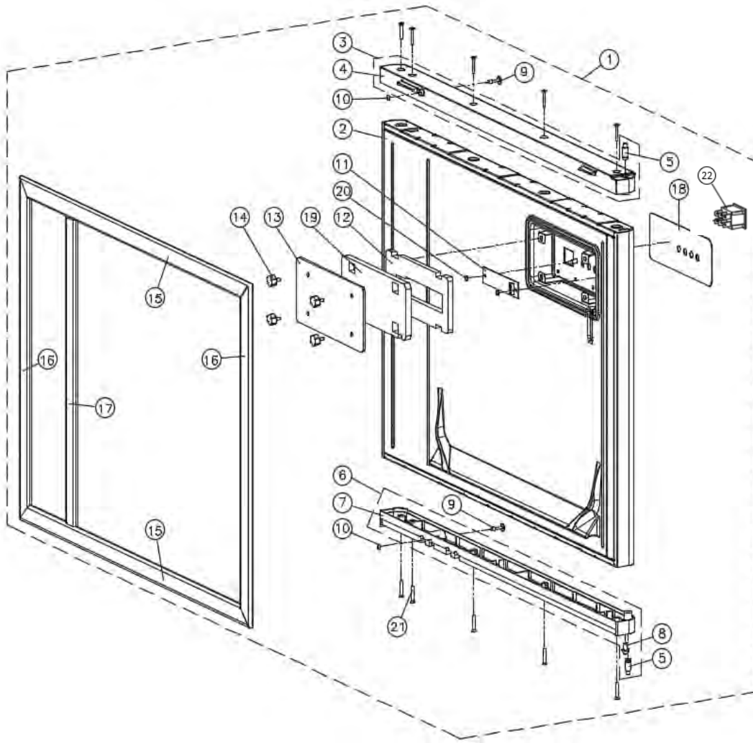
[ FRONT PANEL ASSY ]
