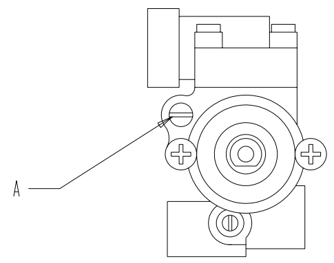
A. Minimum adjustment screw Figure 7 - Safety valve
