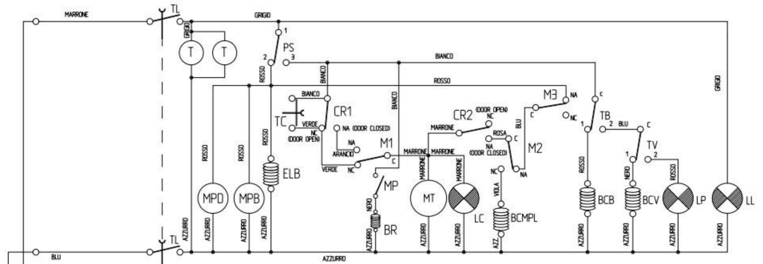
TIMER DIAGRAM
