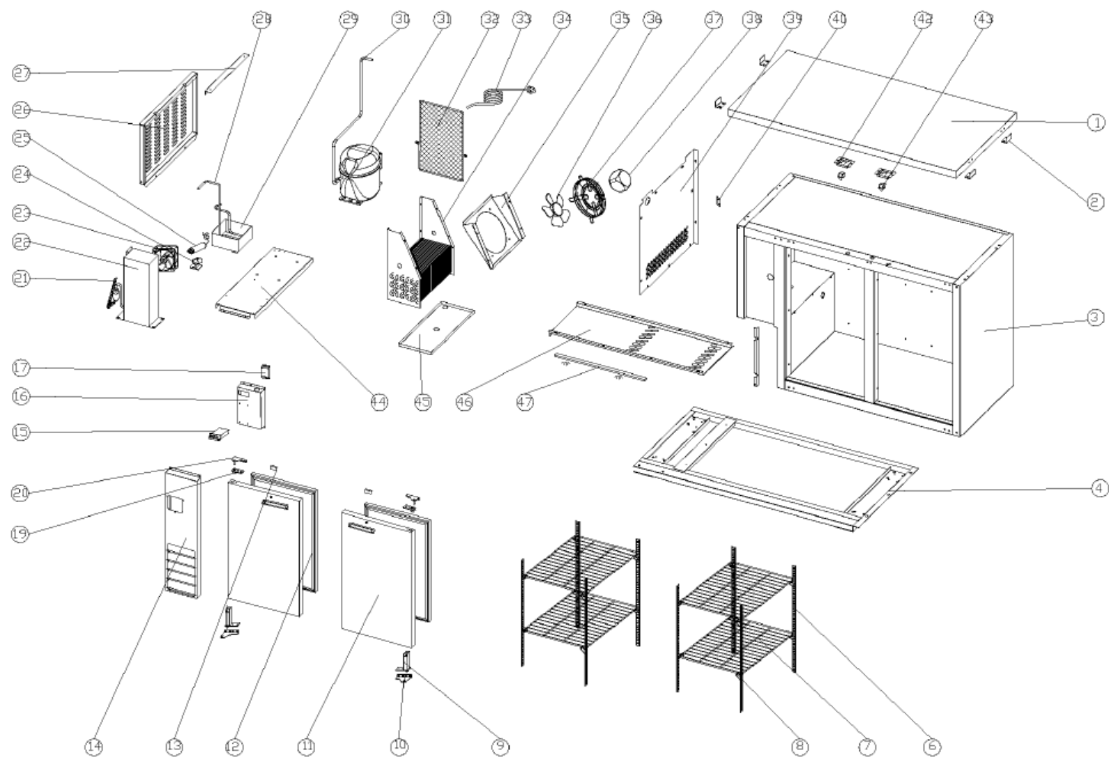
KELVINATOR COMMERCIAL KCHBB48SS - exploded view
