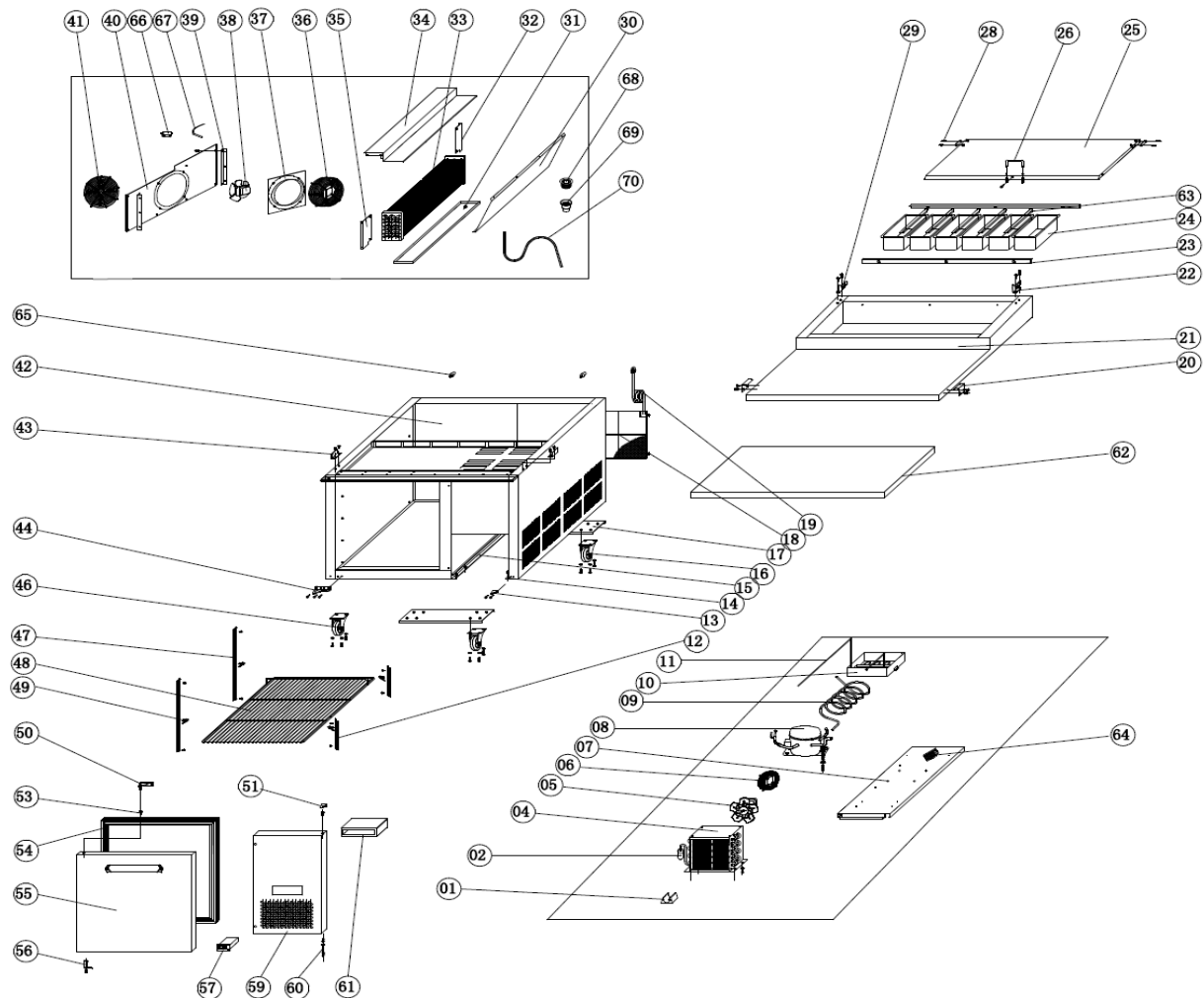
EXPLODE OF KCHPT50.6
